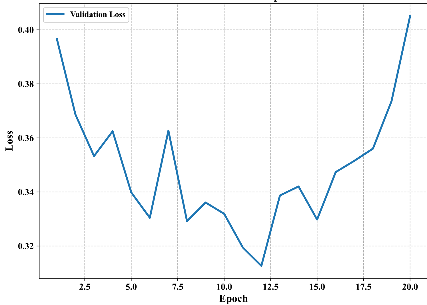
Validation Loss vs Epoch
